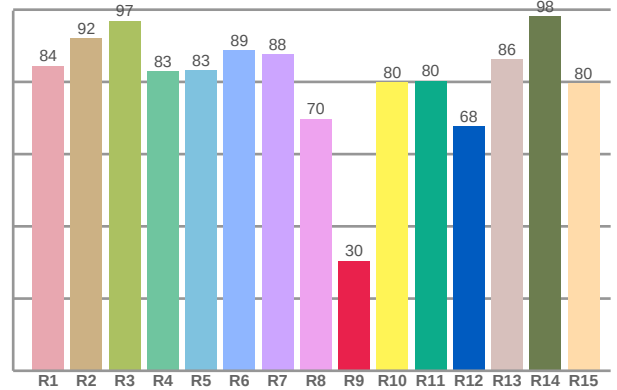
CRI: 85.7 (R1-R8)
