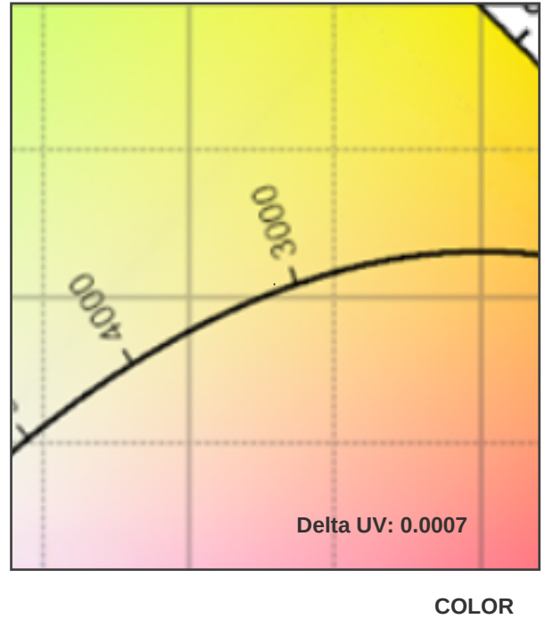
CRI: 85.7 (R1-R8)
